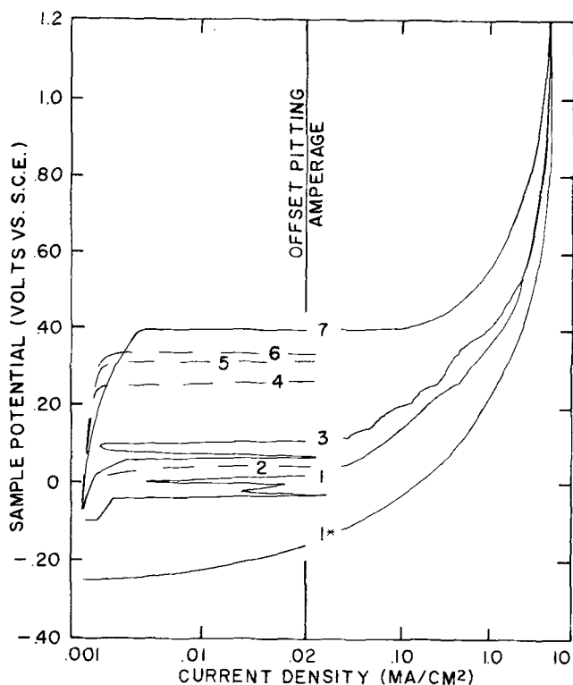
Fig. 1—Anodic polarization data for 18 pct Cr, 18 pct Mn stainless steels of increasing nitrogen content. Offset pitting potential has been determined by the intersection of the anodic polarization data with the offset pitting amperage. 1* indicates data for Alloy 1 after thermal ferritization.
