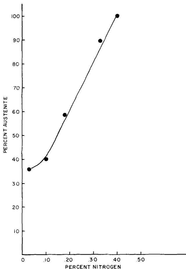
Fig. 3—The effect of nitrogen additions upon the relative amount of austenite observed in 18 pct Cr, 18 pct Mn stainless steels.
